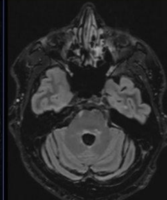
Multiple Sclerosis
